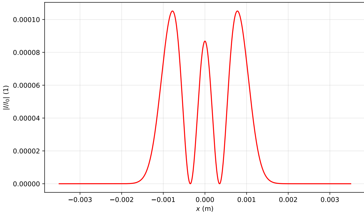
Intensity profile I(x, y = 0, z = 0.159)/I_0 , P_{in}=6.0P_{cr} , artificial time
